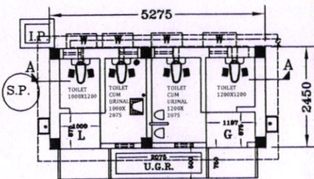
SECTIONAL PLAN
