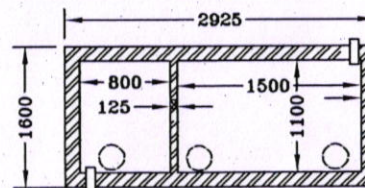
SECTIONAL PLAN OF SEPTIC TANK (20 users)
