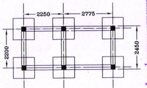
LAYOUT OF COLUMN AND FLOOR BEAM
