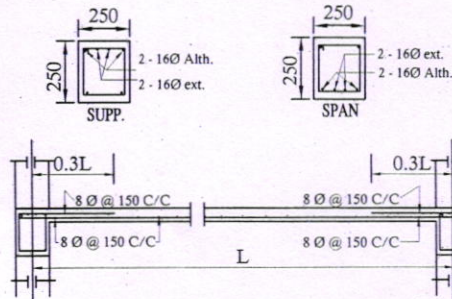
Details Of R.C.C Roof Slab & Beam
