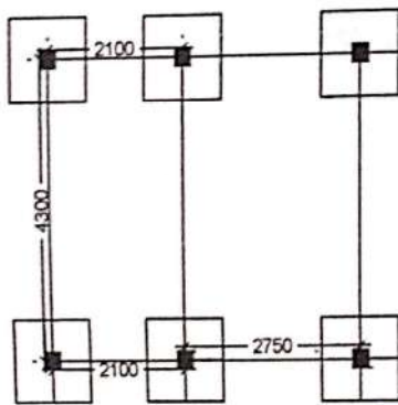
LAYOUT PLAN
