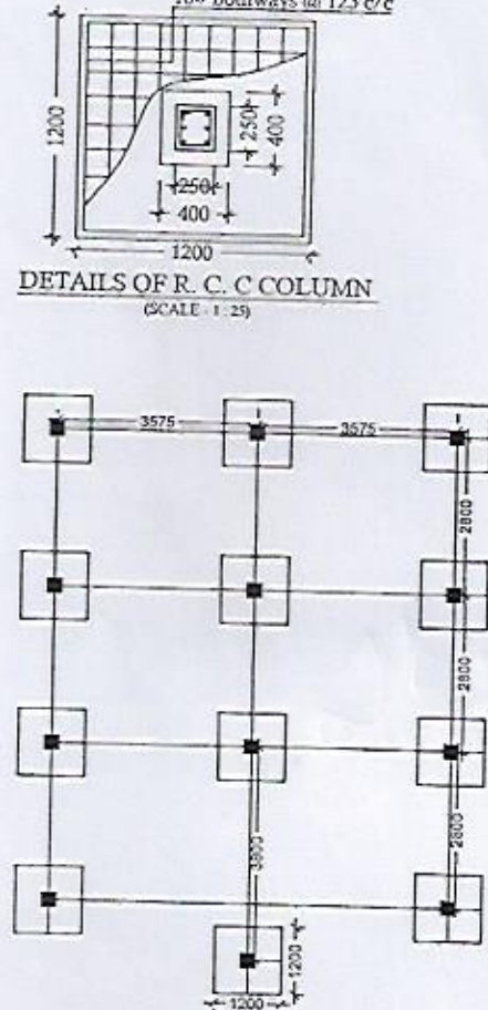
LAYOUT PLAN
