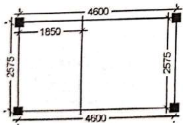
LAYOUT PLAN
