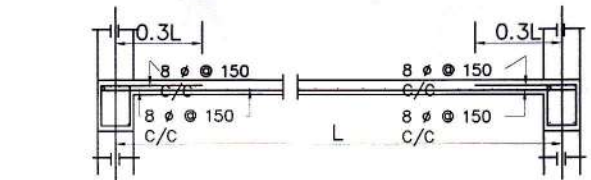
Details Of R.C.C Roof Slab & Beam
