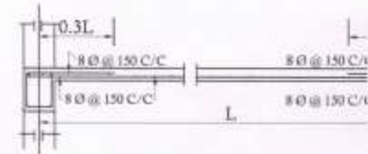
Details Of R.C.C Roof Slab
