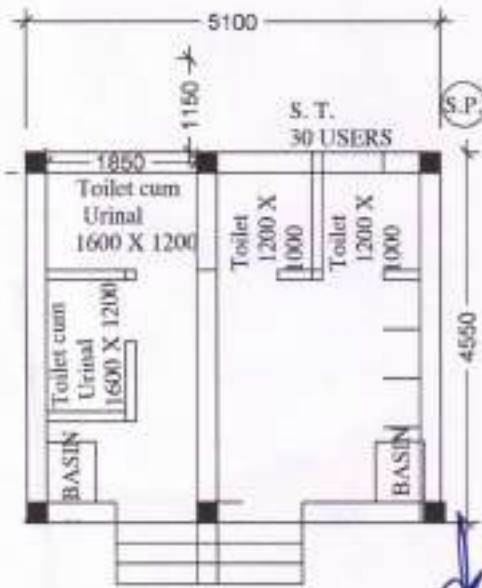
PLAN
