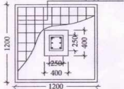
DETAILS OF R. C. C COLUMN
