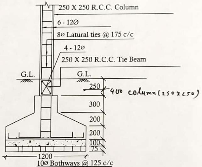
DETAILS OF R. C. C COLUMN (SCALE - 1 : 25)
