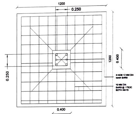
PLAN OF RCC FOUNDATION (1:25)
