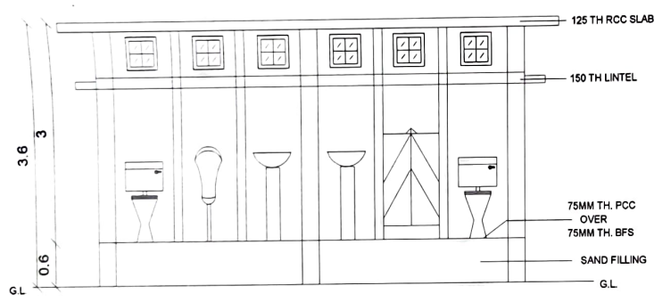
CROSS SECTIONAL VIEW AT X-Y
