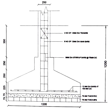
CROSS SECTION OF RCC FOUNDATION (1:25)
