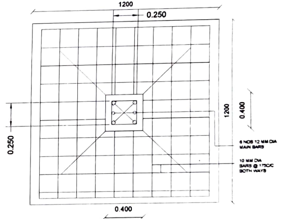
PLAN OF RCC FOUNDATION (1:25)
