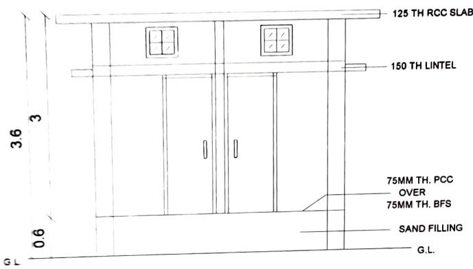
CROSS SECTIONAL VIEW AT X-Y
