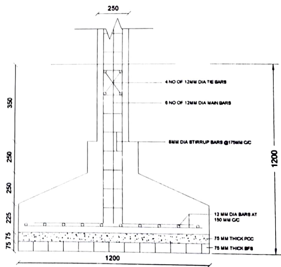
CROSS SECTION OF RCC FOUNDATION (1:25)
