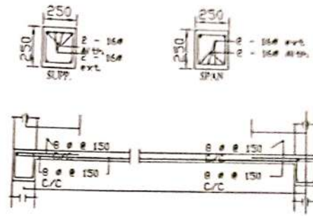
Details Of R.C.C Roof Slab & Beam (SCALE - 1 : 25)
