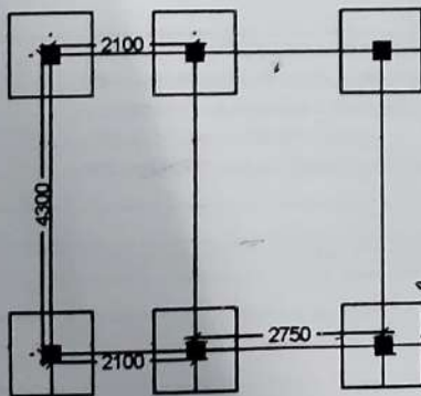
LAYOUT PLAN
