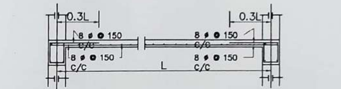
Details Of R.C.C Roof Slab & Beam (SCALE - 1 : 25)
