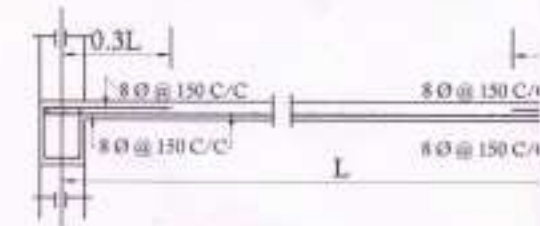
Details Of R.C.C Roof Slab (SCALE - 1 : 25)
