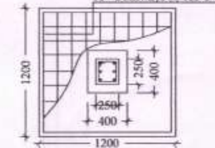
DETAILS OF R. C. C COLUMN (SCALE - 1 : 25)
