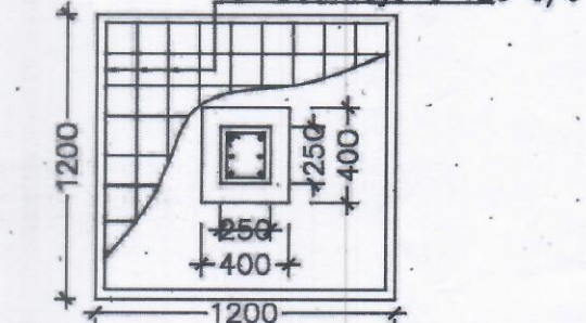
DETAILS OF R. C. C COLUMN
