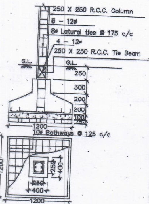
DETAILS OF R. C. C COLUMN (SCALE - 1 : 25)
