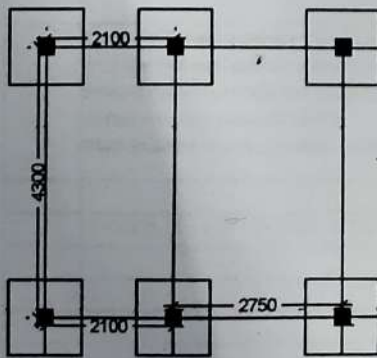
LAYOUT PLAN
