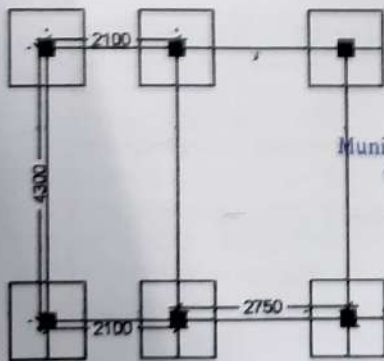
LAYOUT PLAN
