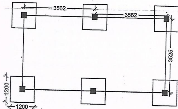
LAYOUT PLAN
