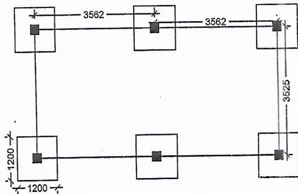
LAYOUT PLAN
