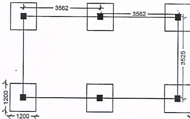
LAYOUT PLAN
