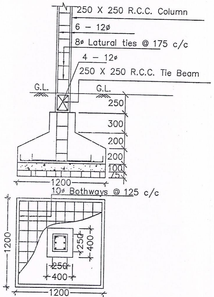
DETAILS OF R. C. C COLUMN
