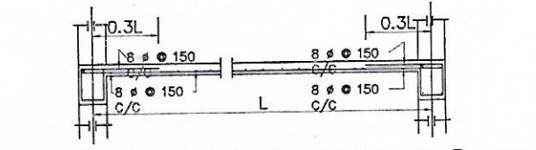
Details Of R.C.C Roof Slab & Beam (SCALE - 1 : 25)
