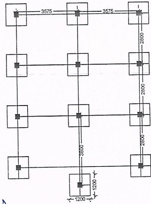
LAYOUT PLAN
