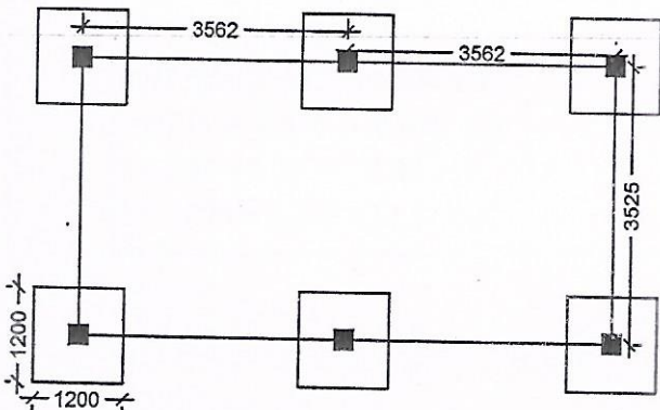
LAYOUT PLAN
