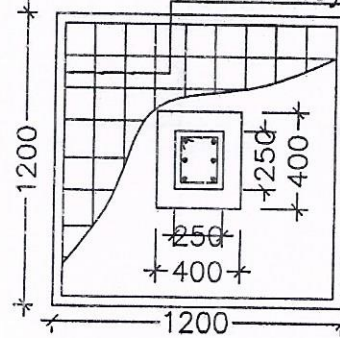
DETAILS OF R. C. C COLUMN (SCALE - 1 : 25)
