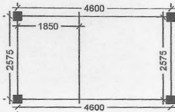
LAYOUT PLAN
