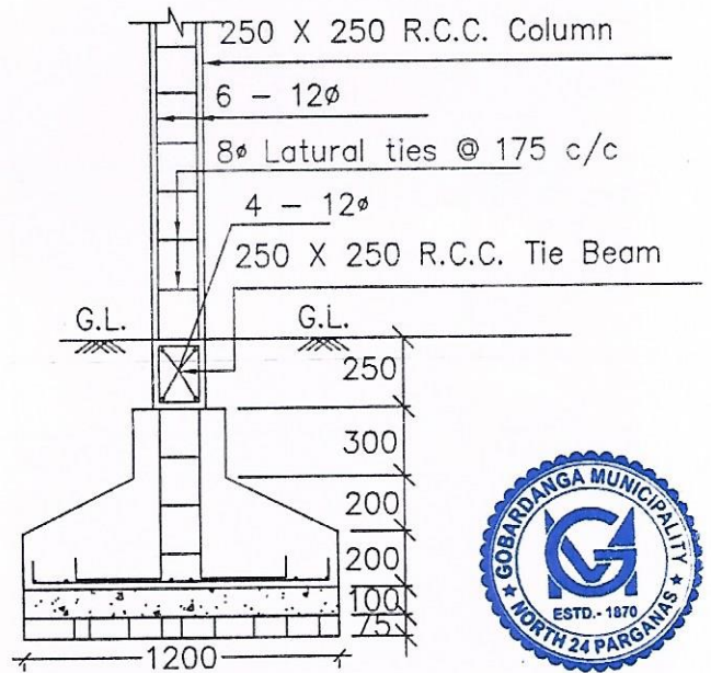
DETAILS OF R. C. C COLUMN
