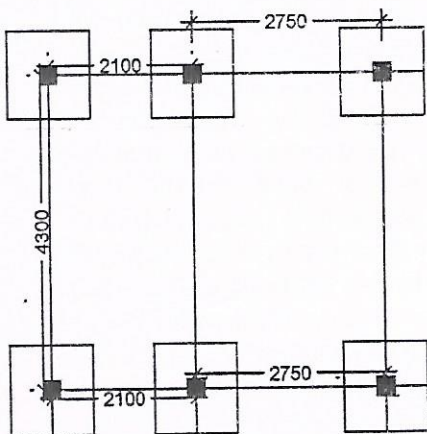
LAYOUT PLAN
