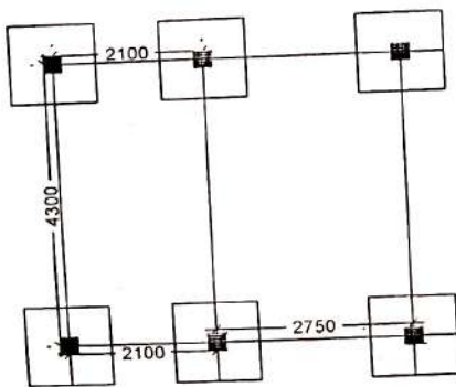
LAYOUT PLAN
