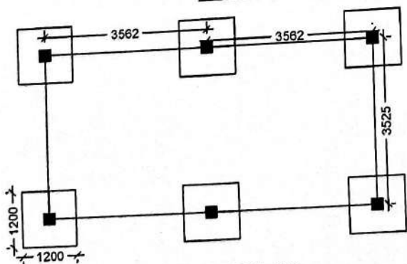
LAYOUT PLAN
