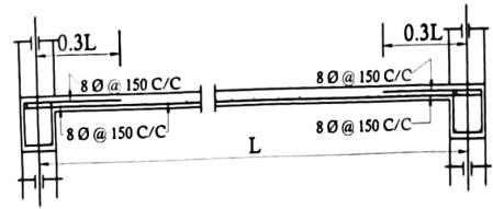
Details Of R.C.C Roof Slab & Beam (SCALE - 1 : 25)
