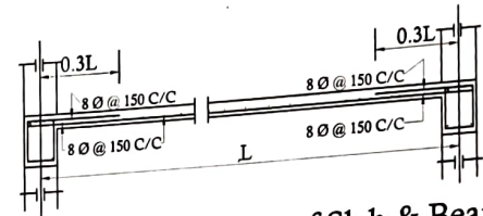
Details Of R.C.C Roof Slab & Beam (SCALE - 1 : 25)
