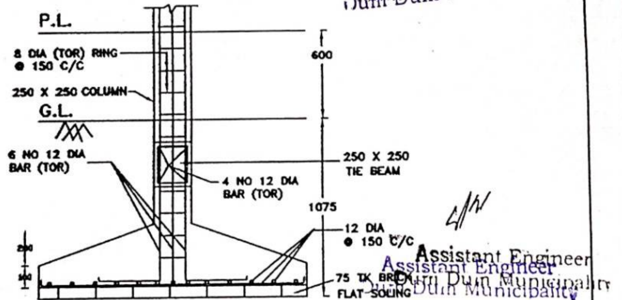
SECTION
