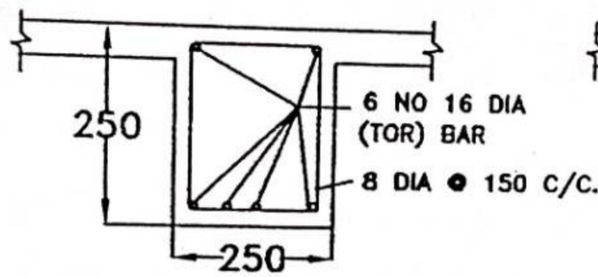
DETAILS OF BEAM AT MID SPAN
