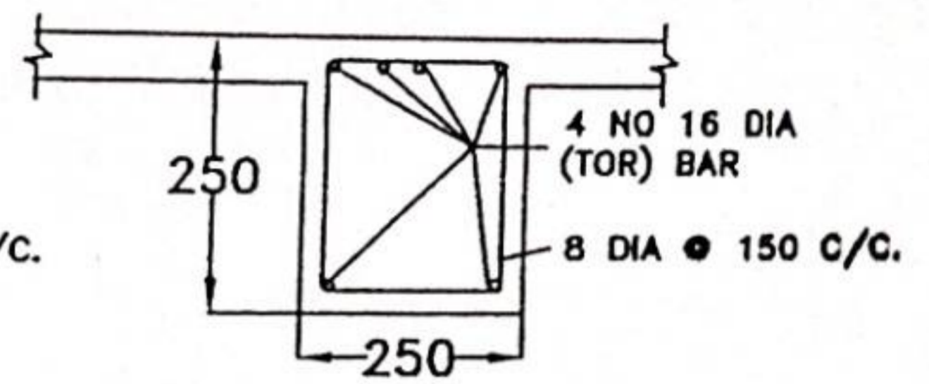
DETAILS OF BEAM AT SUPPORT
