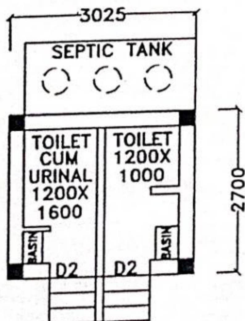
PLAN
