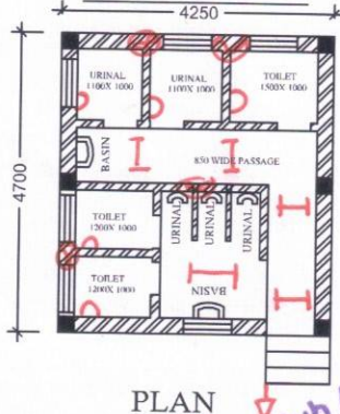
LAYOUT PLAN
