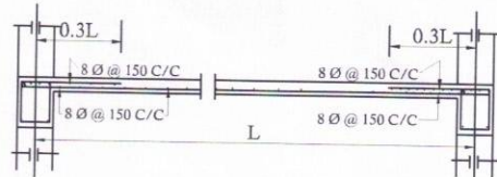
Details Of R.C.C Roof Slab & Beam(Existing)
