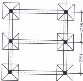
LAYOUT PLAN
