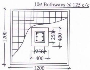
DETAILS OF R. C. C COLUMN(EXISTING)
