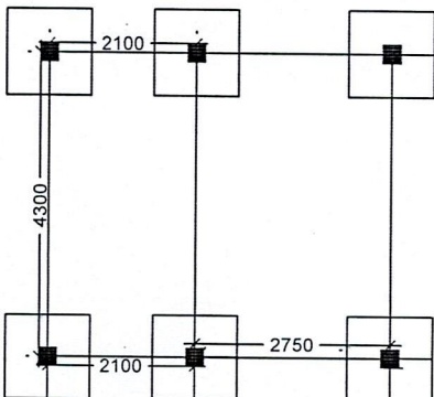
LAYOUT PLAN
