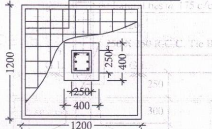
DETAILS OF R. C. C COLUMN(For Extended Portion)
