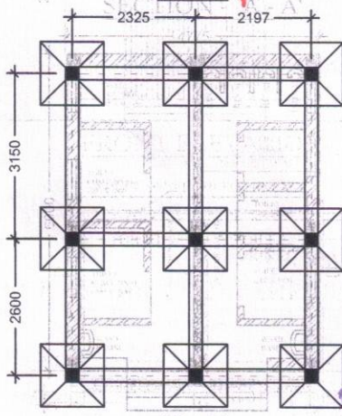
LAYOUT PLAN
