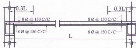
Details Of R.C.C Roof Slab & Beam(Partly Extended)
