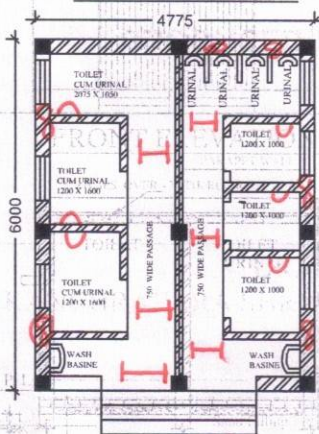
PLAN
