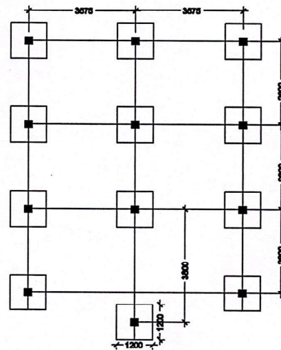
LAYOUT PLAN
