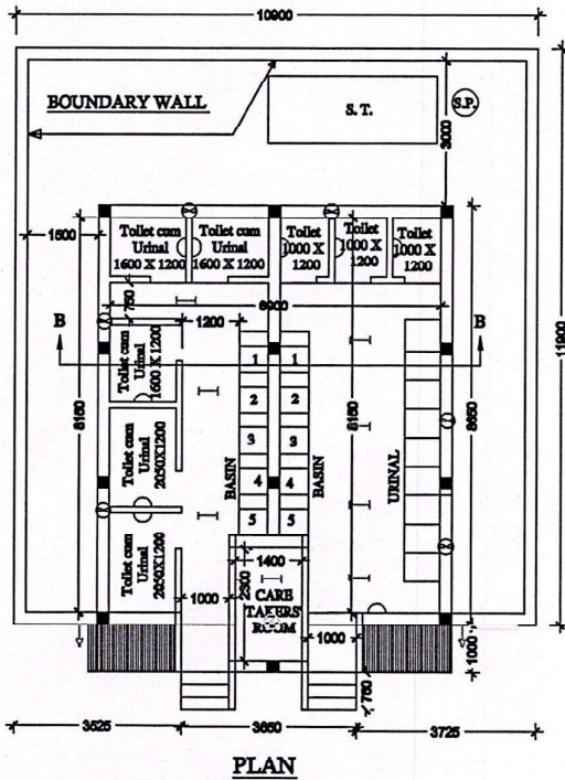
PLAN
