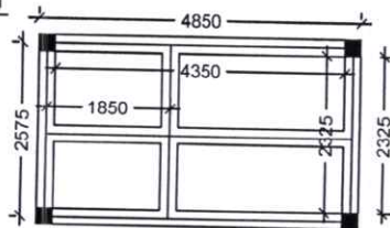
LAYOUT ROOF BEAM PLAN
