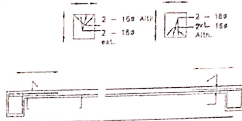
Details Of R.C.C Roof Slab & Beam (SCALE - 1 : 25)
