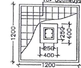
DETAILS OF R. C. C COLUMN (SCALE - 1 : 25)
