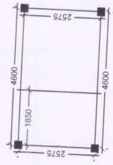
LAYOUT PLAN
