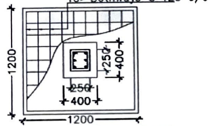
DETAILS OF R. C. C COLUMN (SCALE - 1 : 25)
