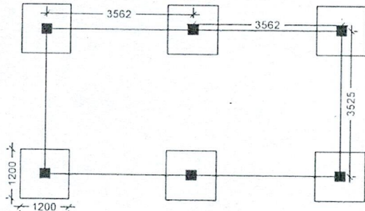
LAYOUT PLAN
