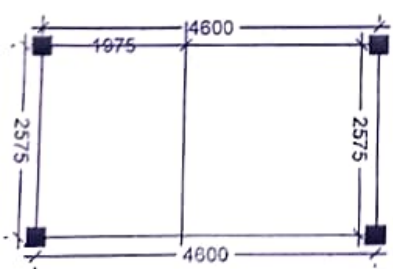
LAYOUT PLAN
