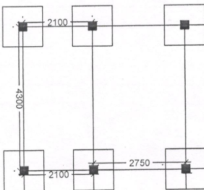
LAYOUT PLAN
