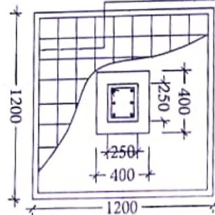
DETAILS OF R. C. C COLUMN (SCALE - 1 : 25)
