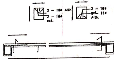
Details Of R.C.C Roof Slab & Beam (SCALE - 1 : 25)
