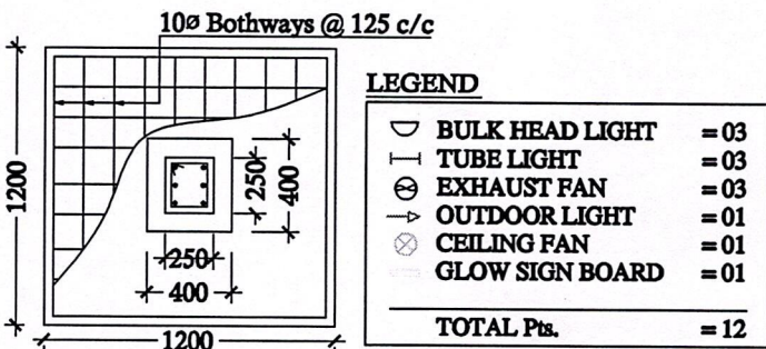
DETAILS OF R. C. C COLUMN (SCALE - 1 : 25)
