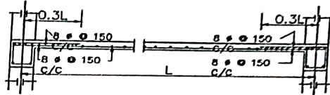
Details Of R.C.C Roof Slab & Beam
