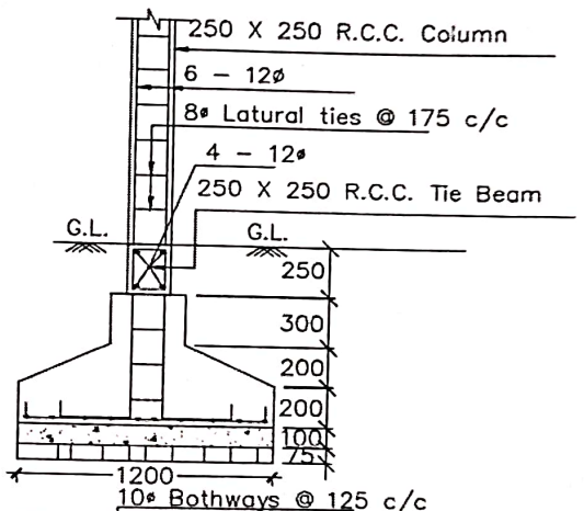
DETAILS OF R. C. C COLUMN (SCALE - 1 : 25)
